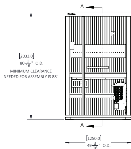
Exterior Front Wall
