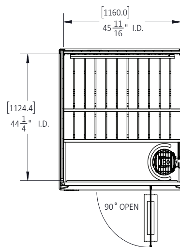
Top Down View w/ Interior Measurements
